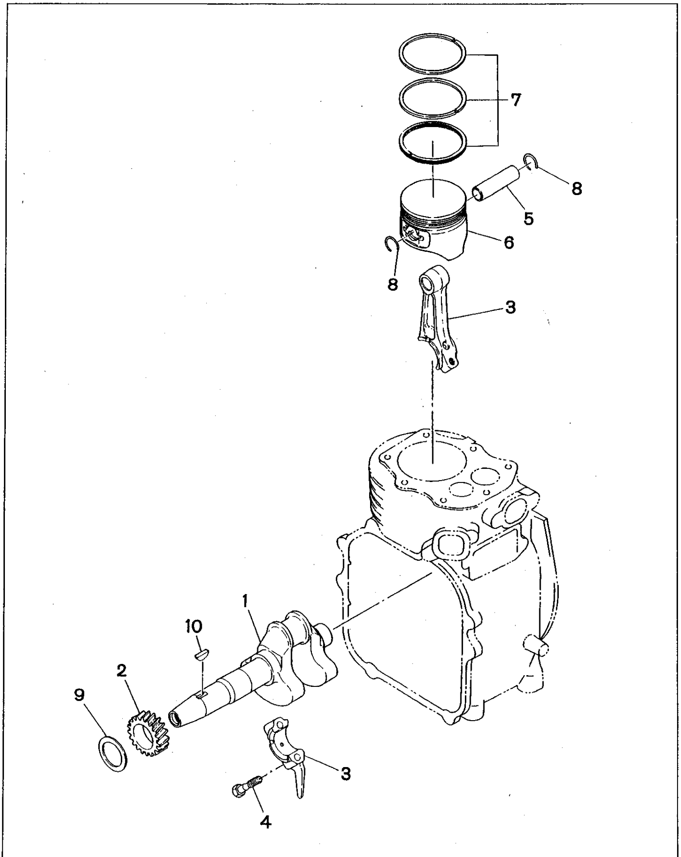
FIG. 6 CRANKSHAFT and PISTON
