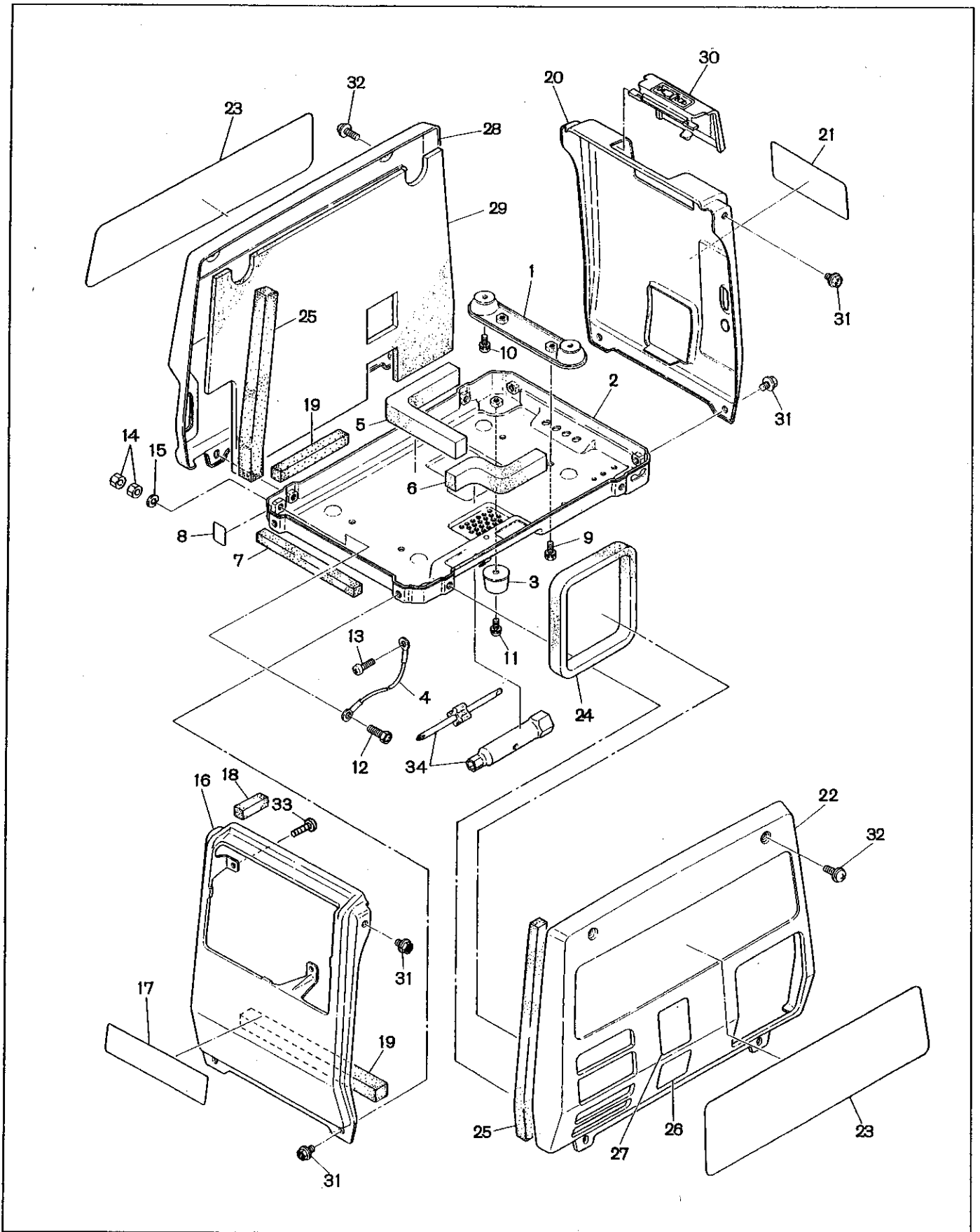
FIG. 2 COVER
