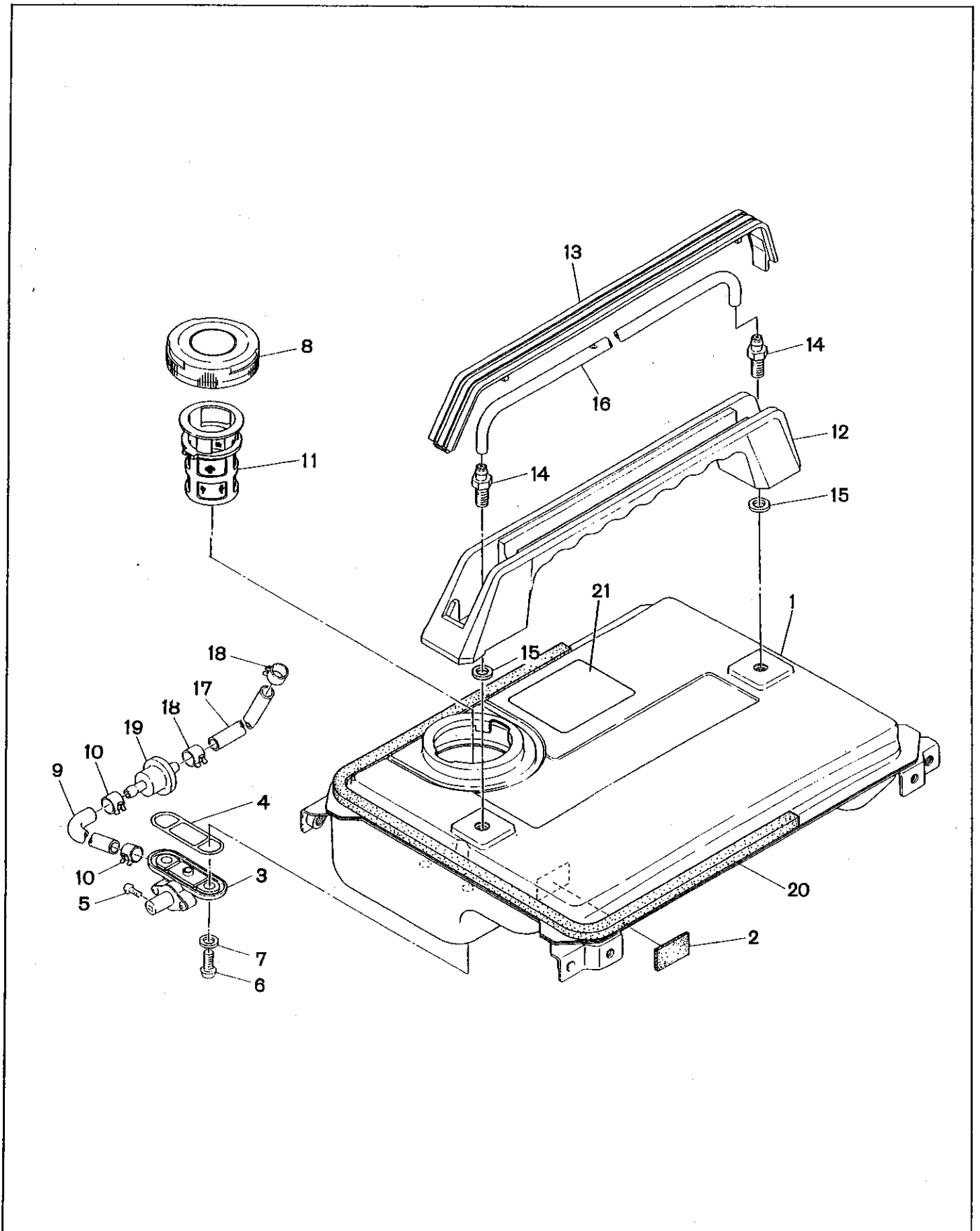
FIG. 4 FUEL TANK
