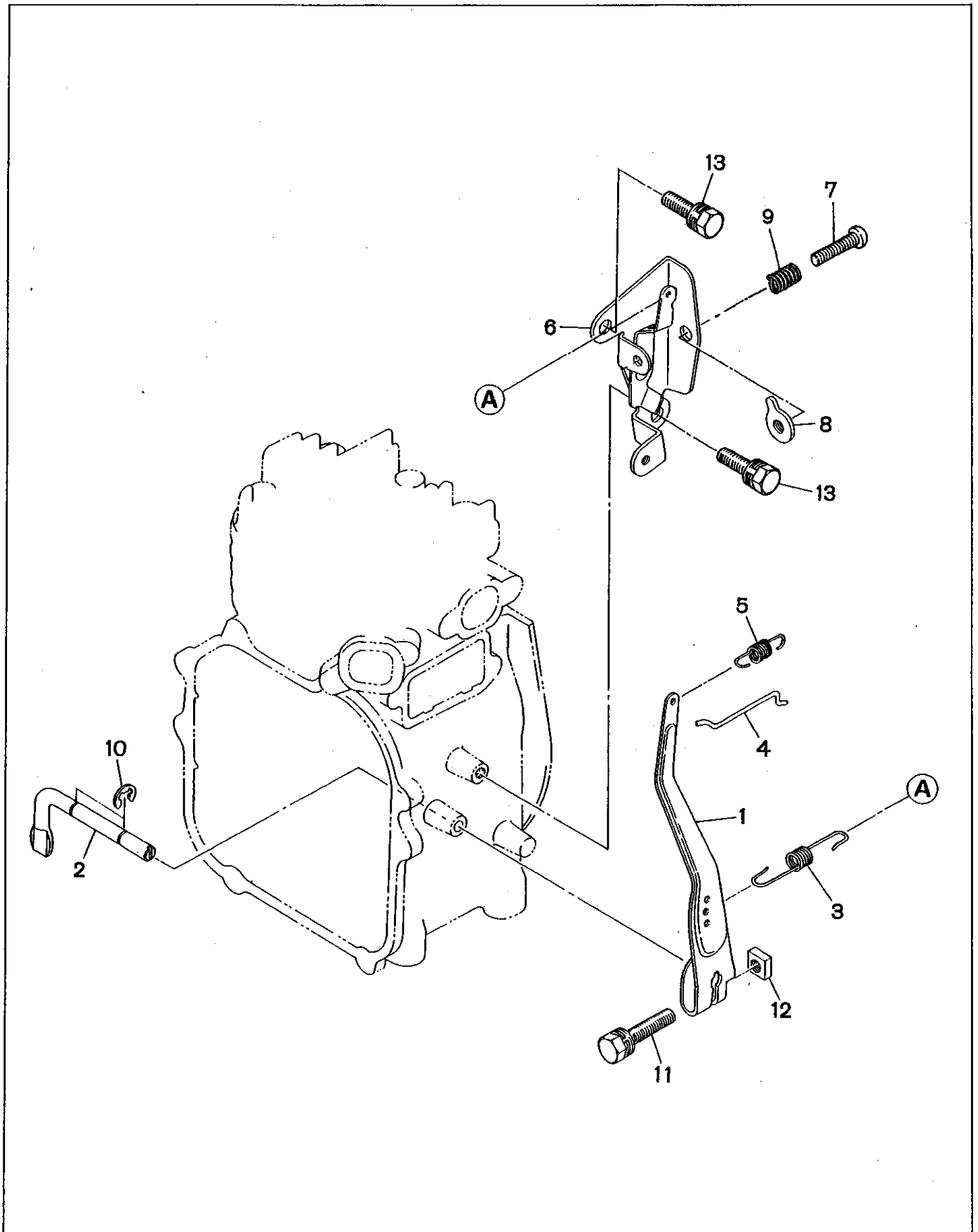
FIG. 8 GOVERNOR, OPERATION
