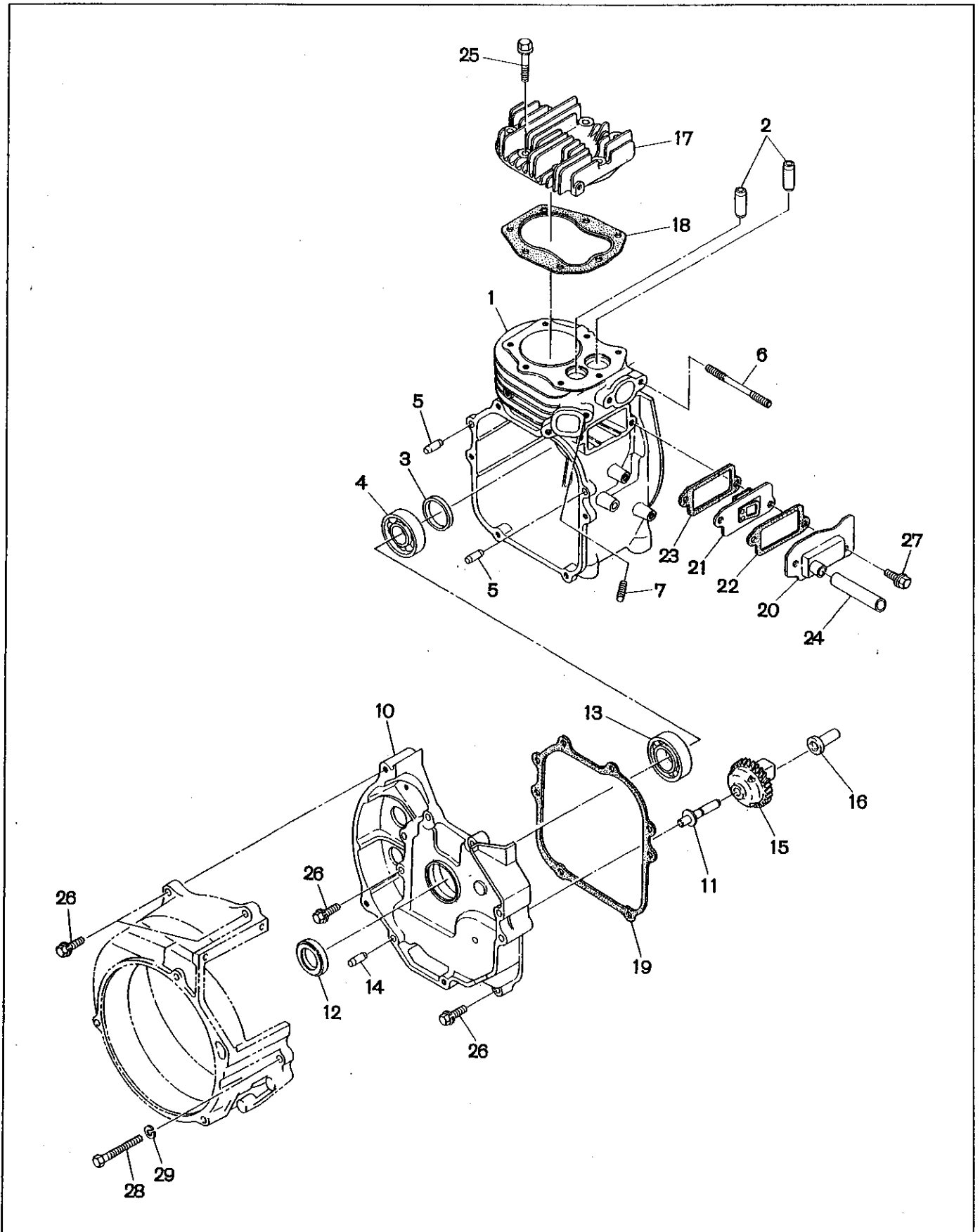
FIG. 5 CRANKCASE
