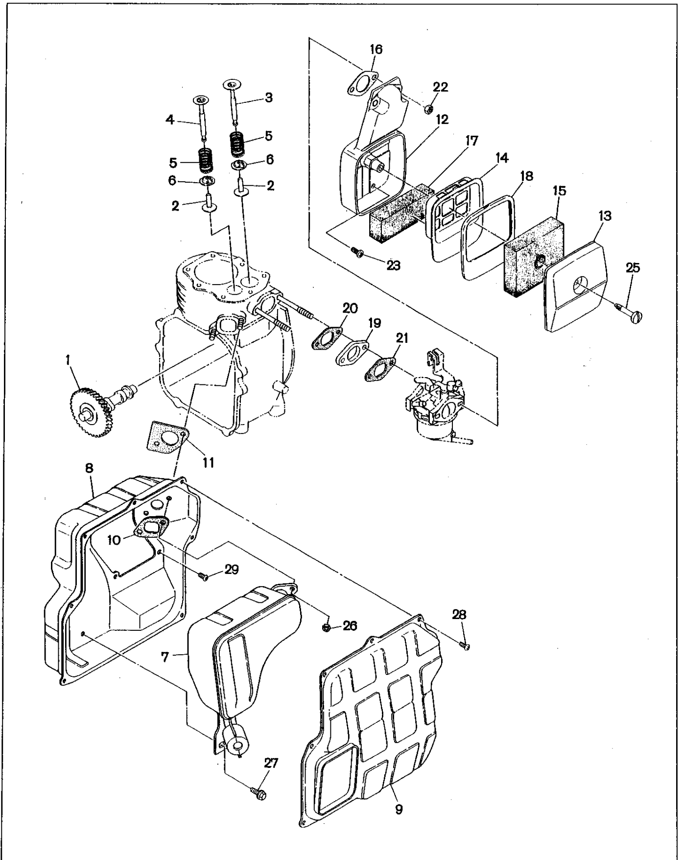
FIG. 7 INTAKE and EXHAUST
