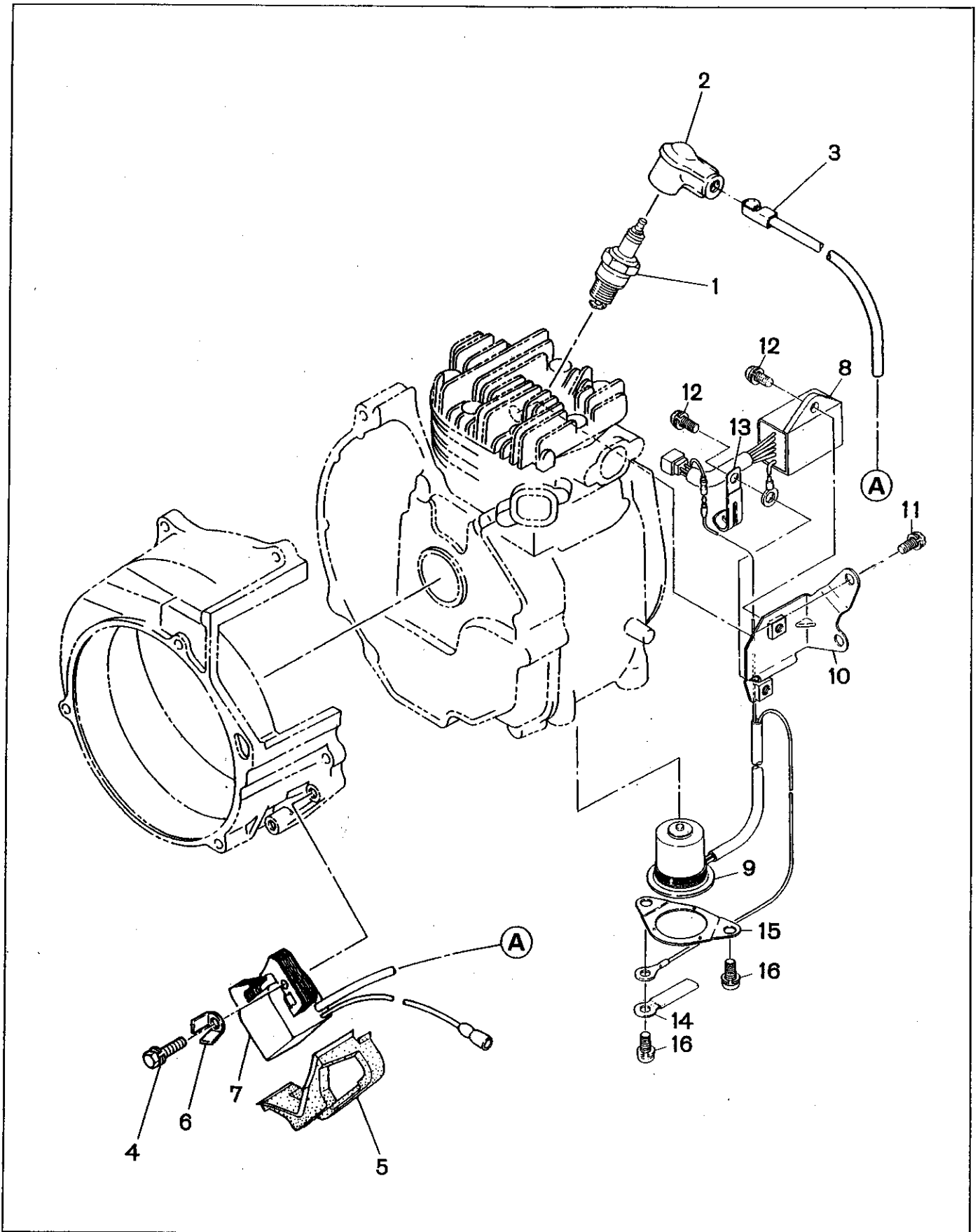
FIG. 11 ELECTRIC DEVICE
