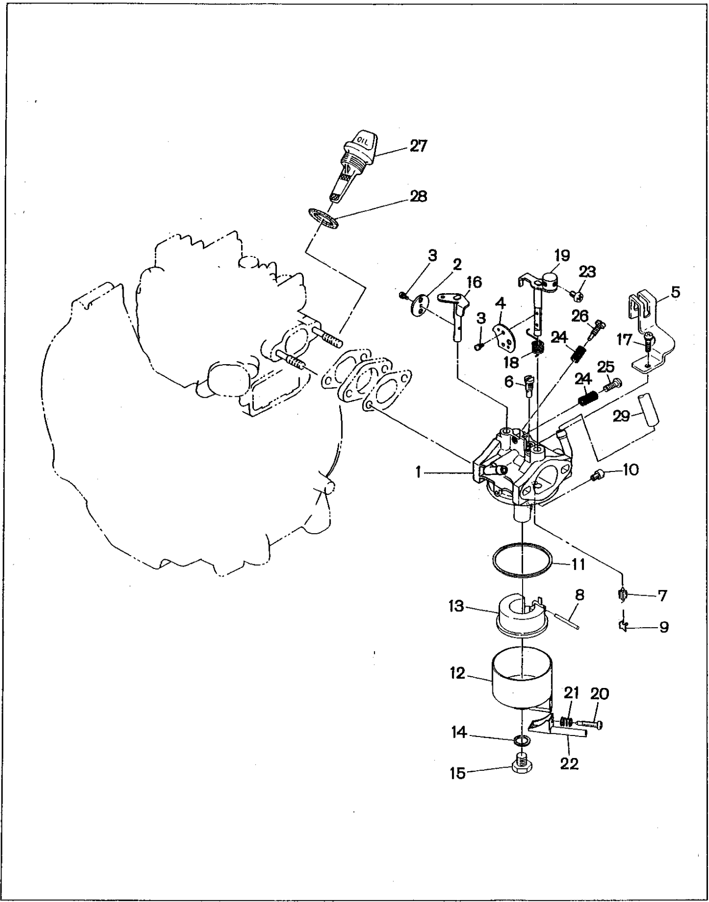
FIG. 10 FUEL LUBRICANT
