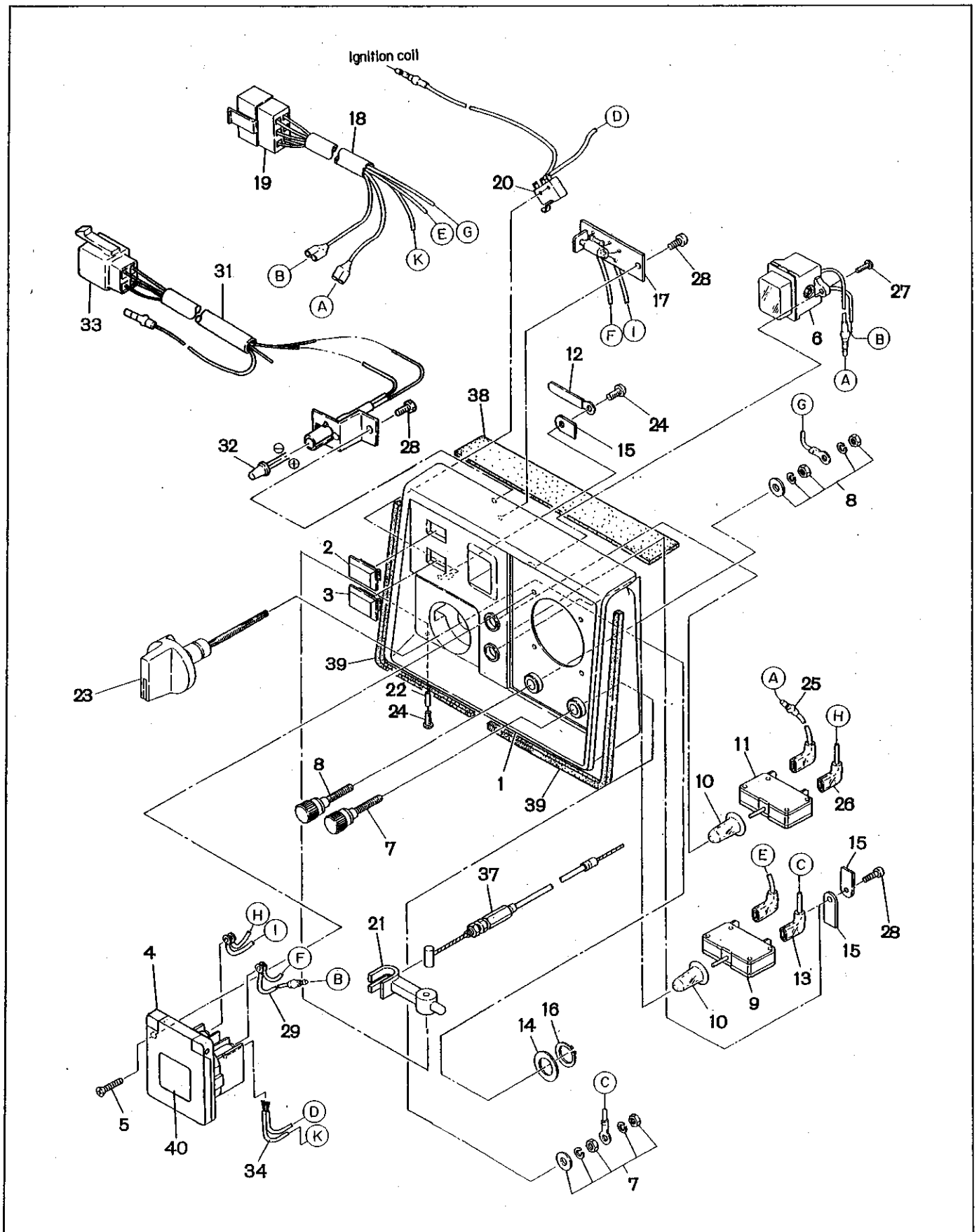
FIG. 3 CONTROL PANEL
