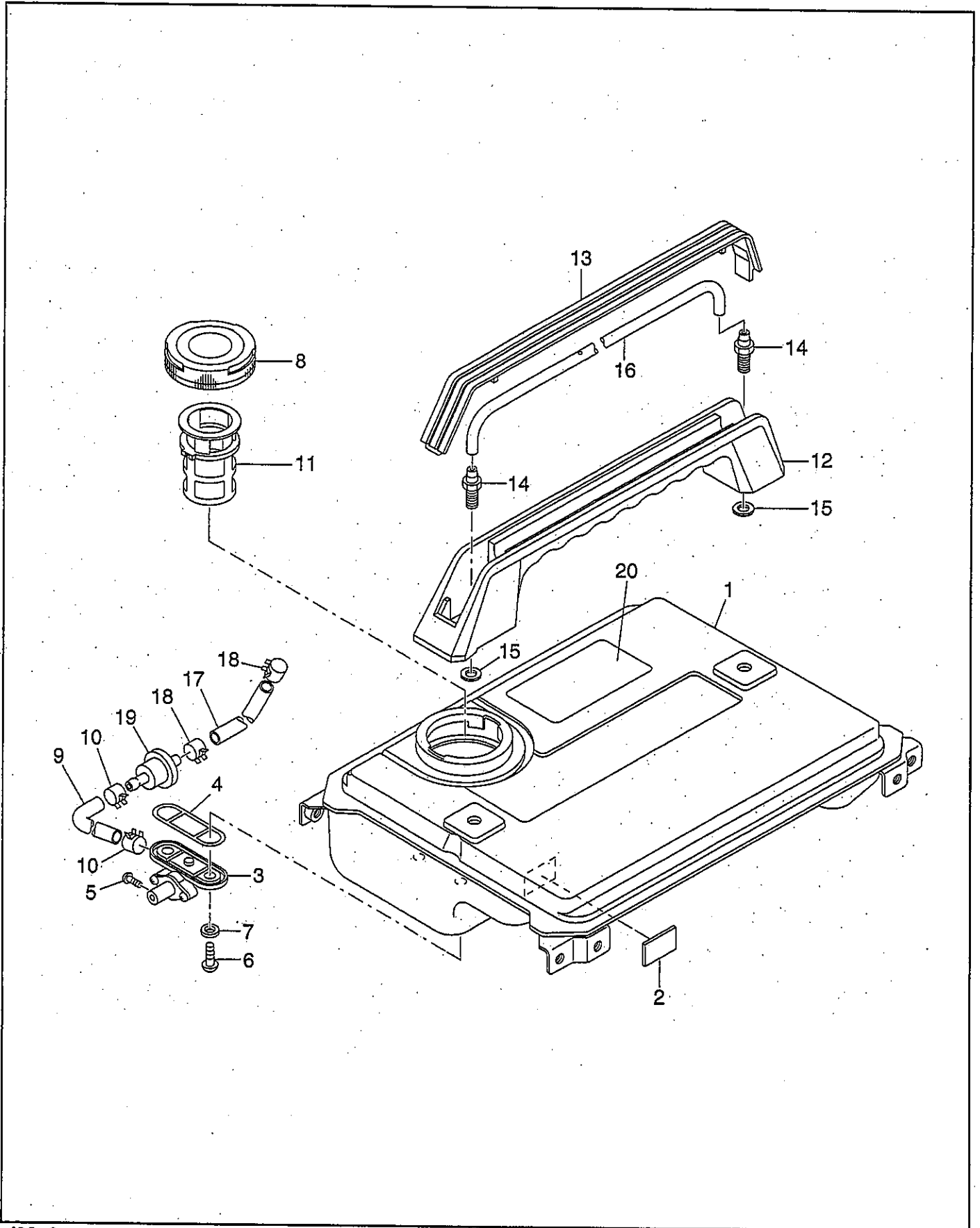
FIG.4 FUEL TANK
