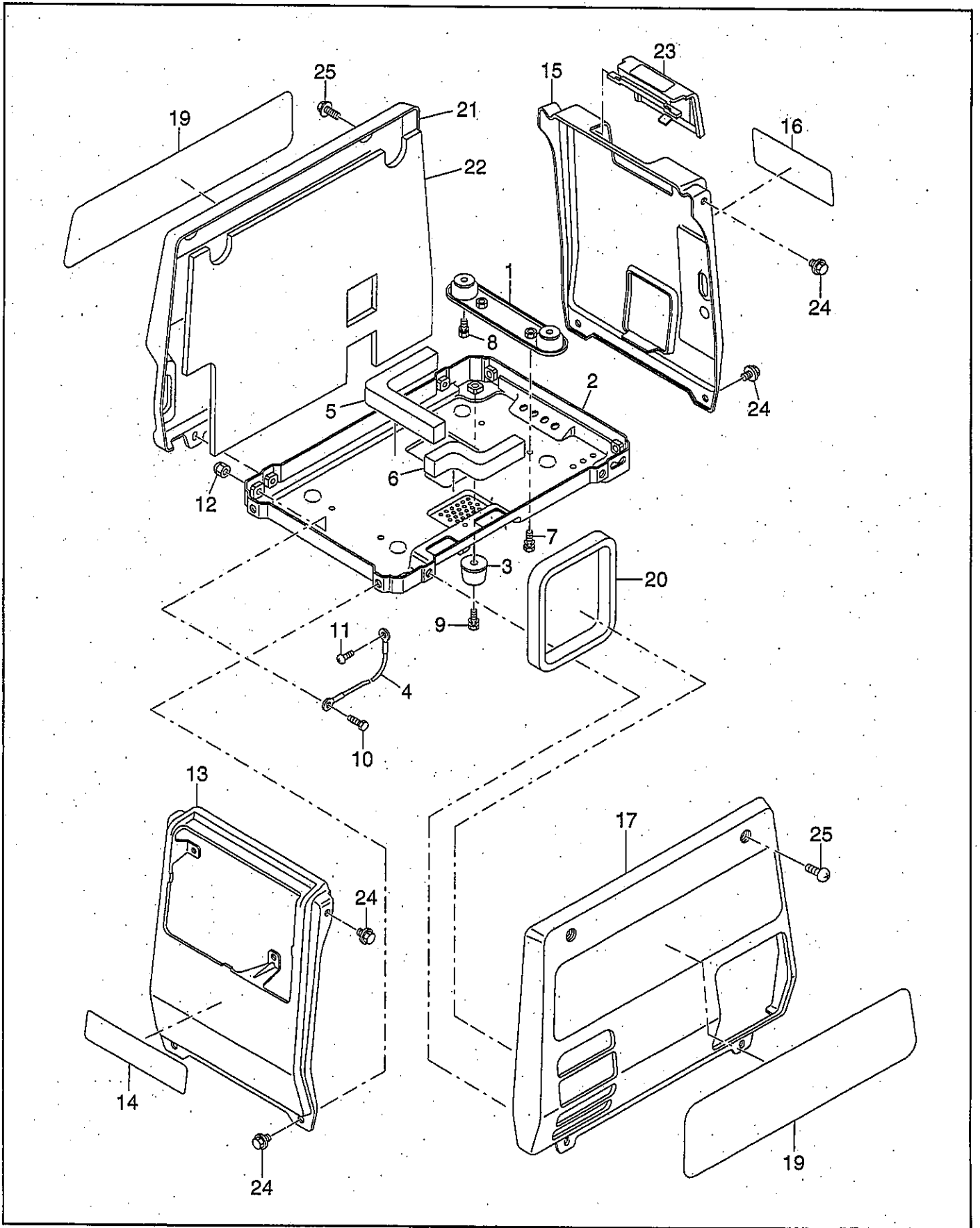
FIG.2 COVER
