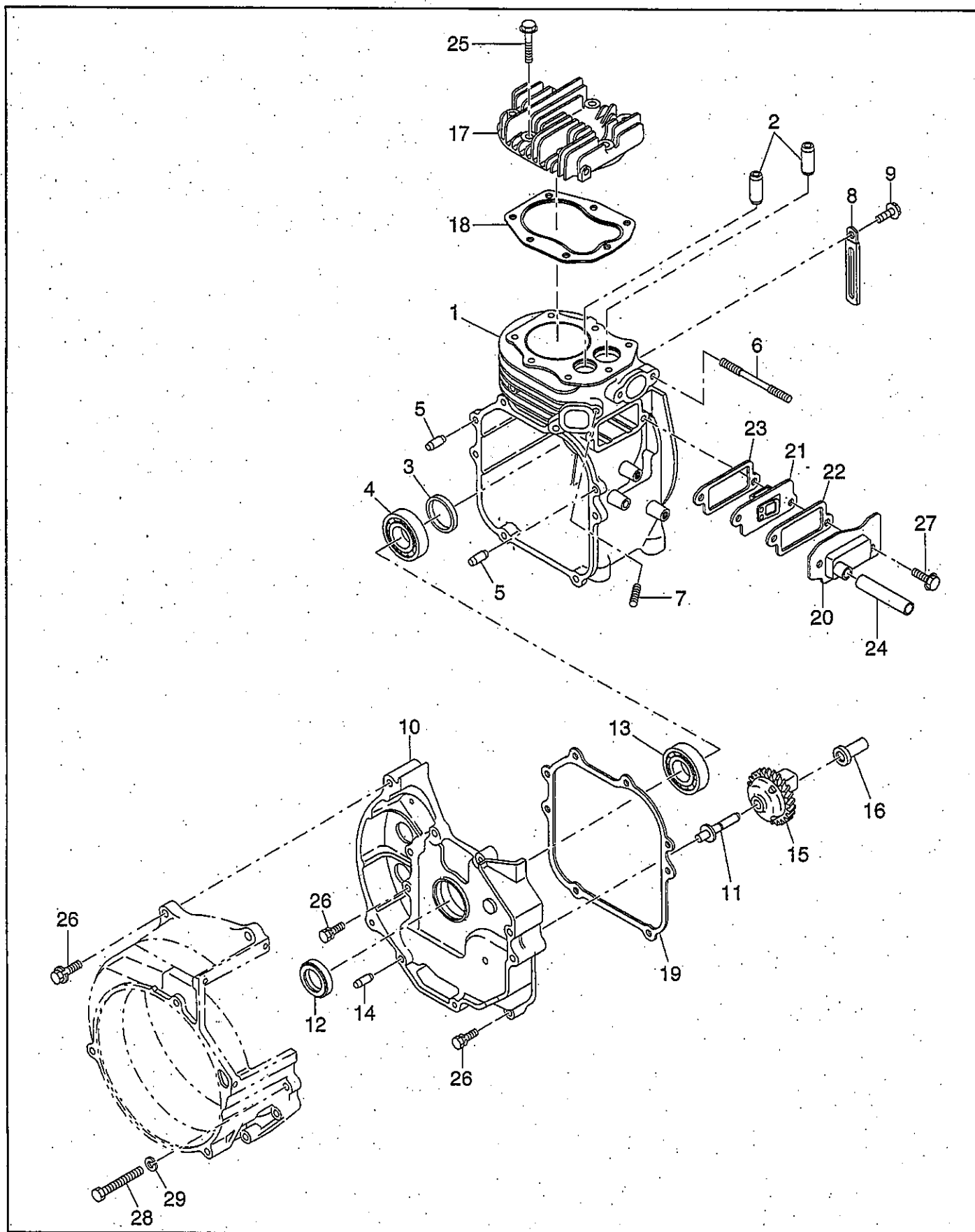
FIG.5 CRANKCASE GROUP
