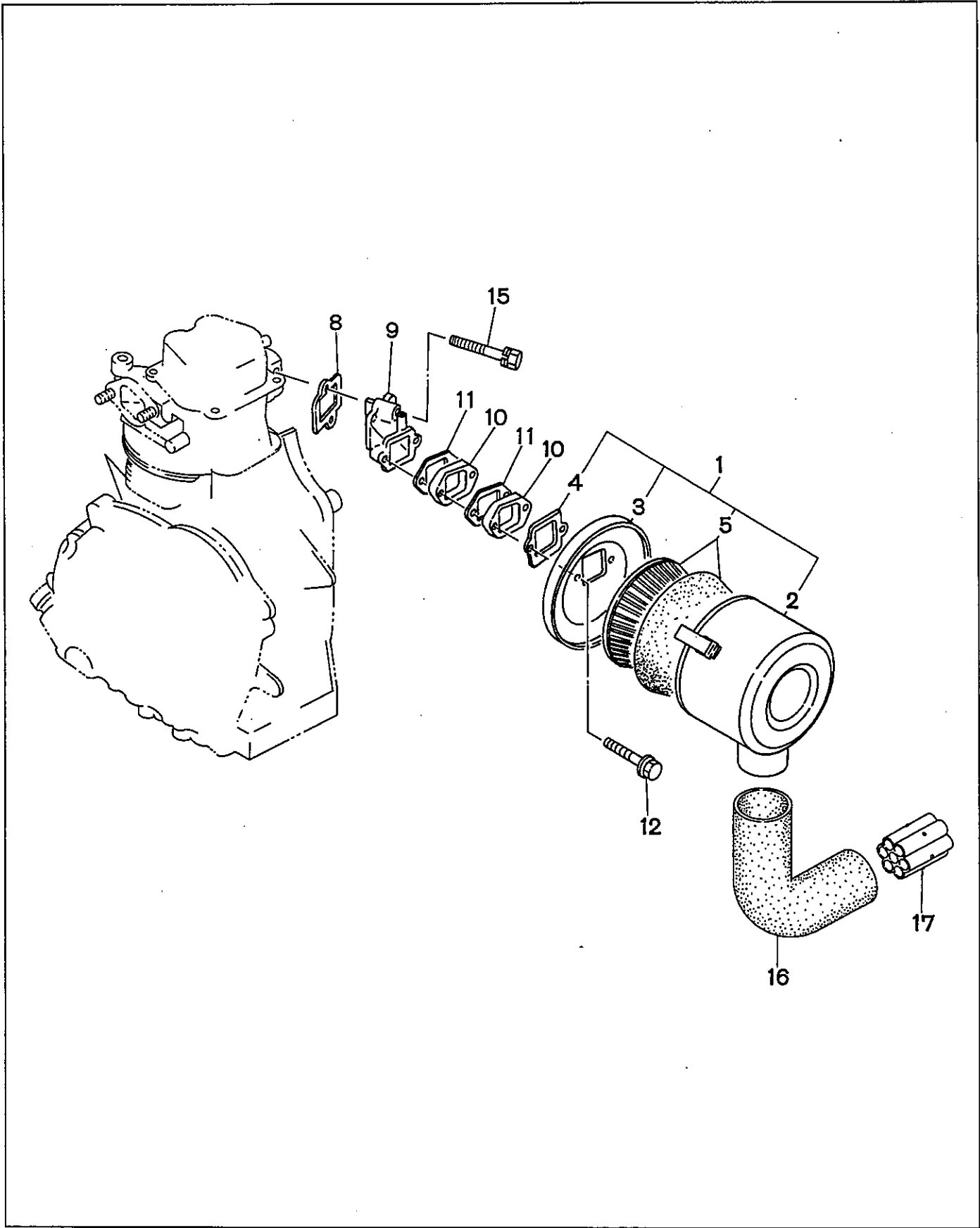
FIG. 11 AIR CLEANER
