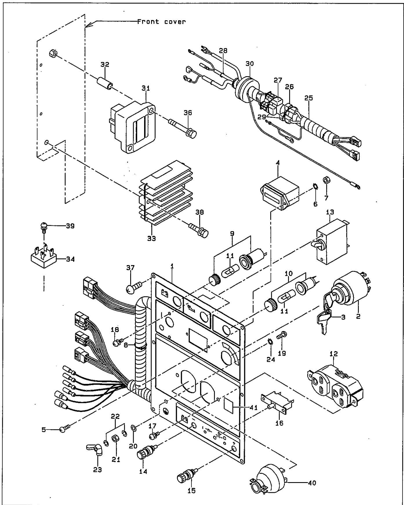
FIG. 3-1 CONTROL PANEL ( STD. 50Hz-220V )
