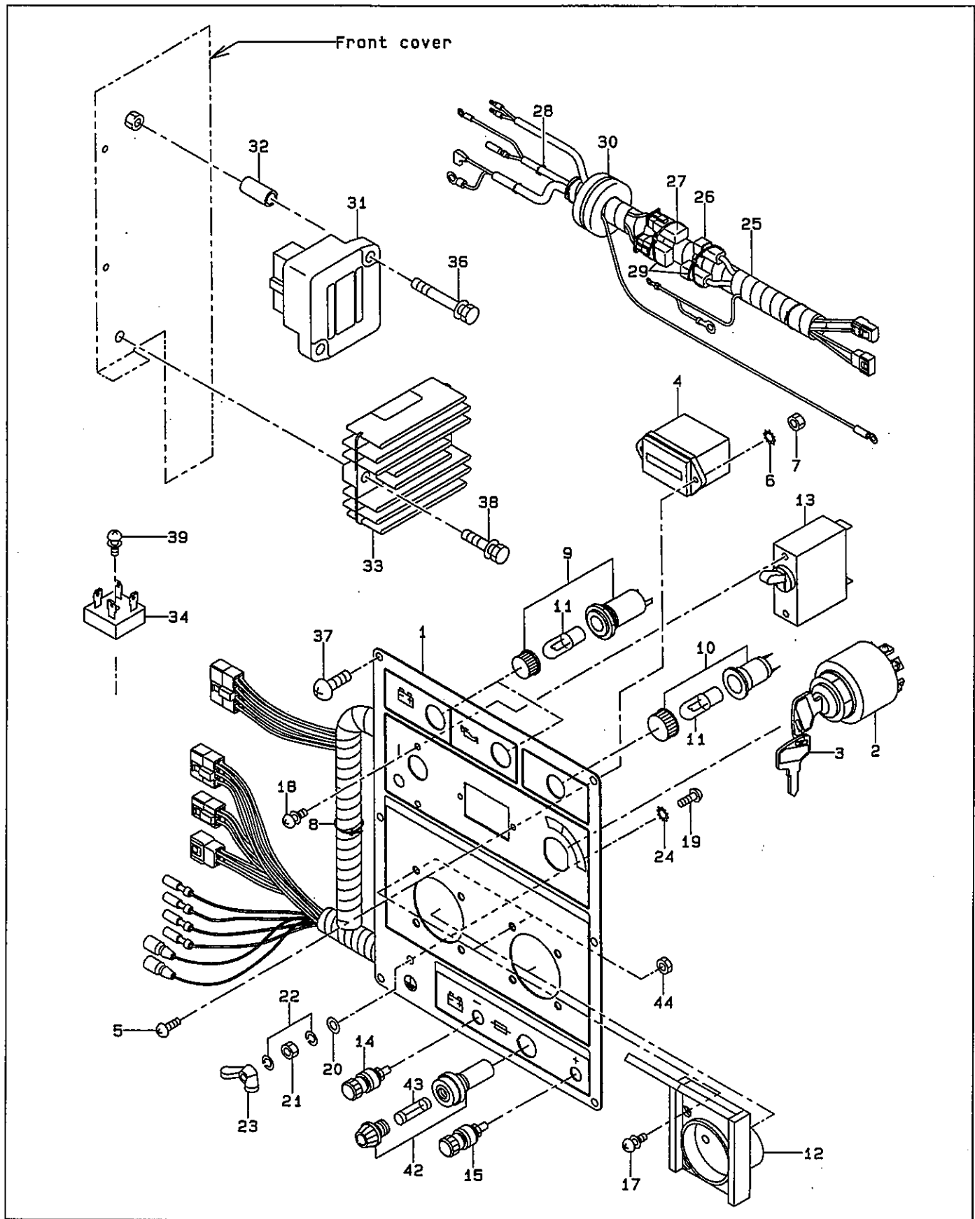
FIG. 3-2 CONTROL PANEL ( FRANCE RECEPTACLE TYPE, 50Hz-230V )
