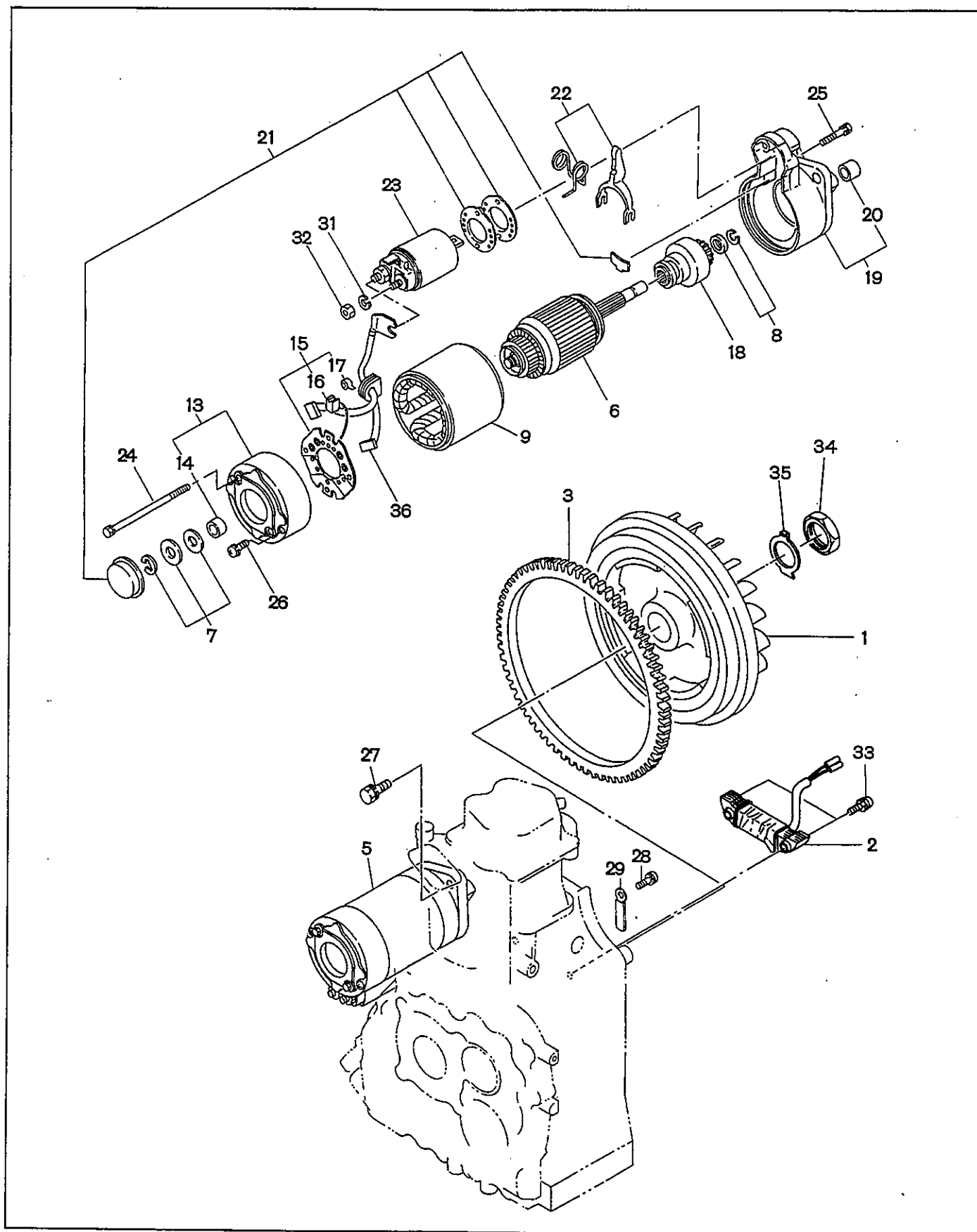
FIG. 15 ELECTRICAL EQUIPMENT
