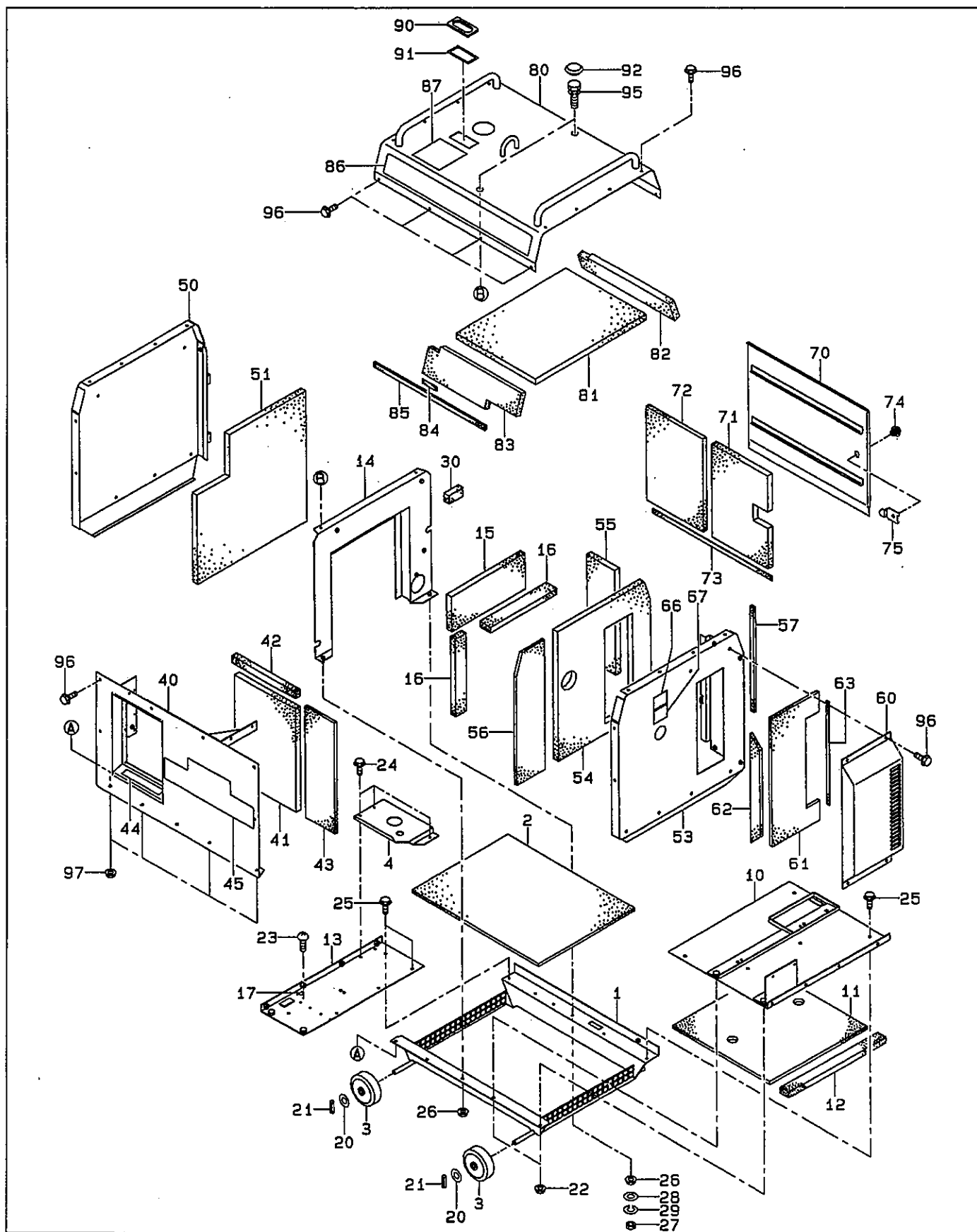
FIG. 2 COVER
