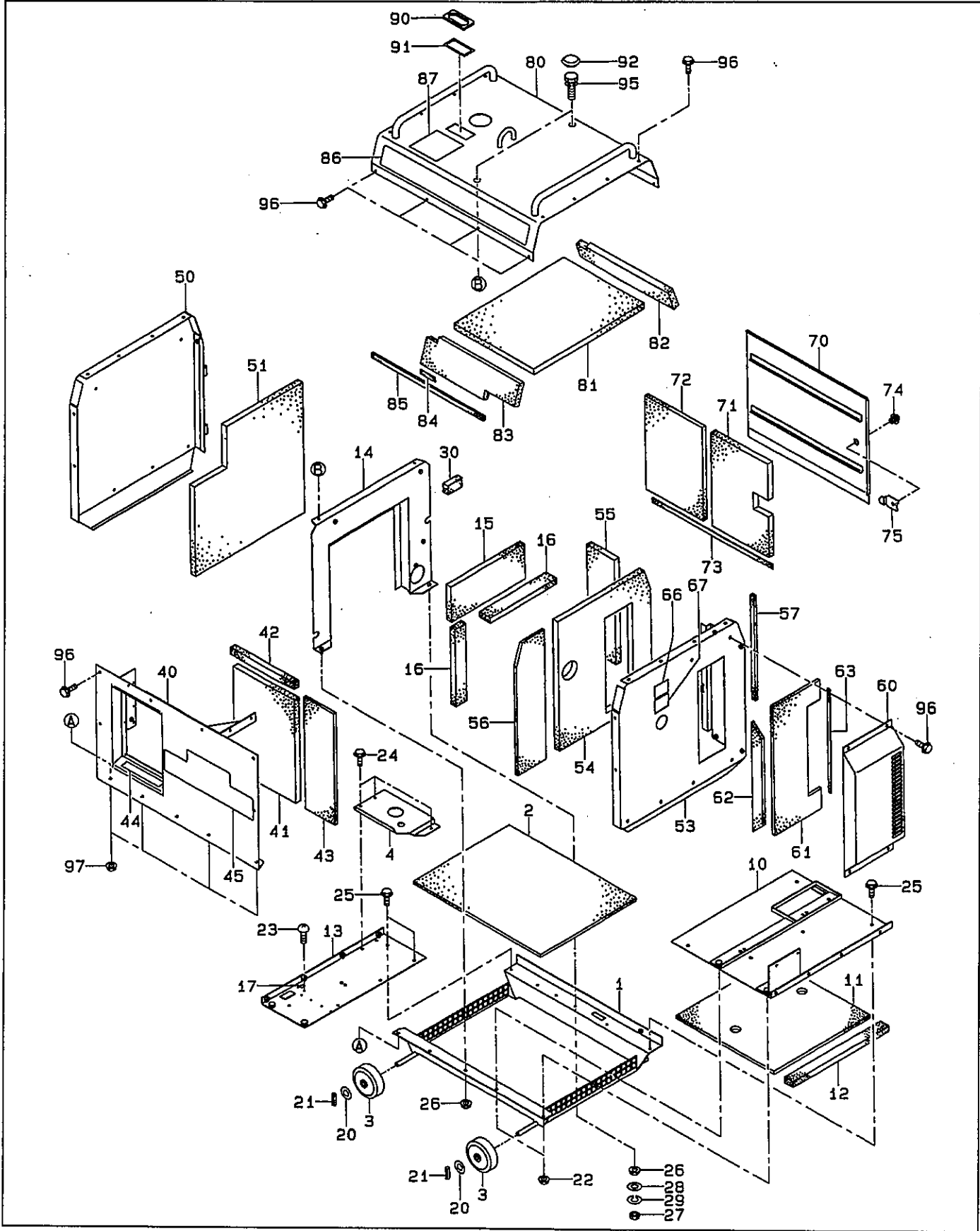
FIG. 2 COVER
