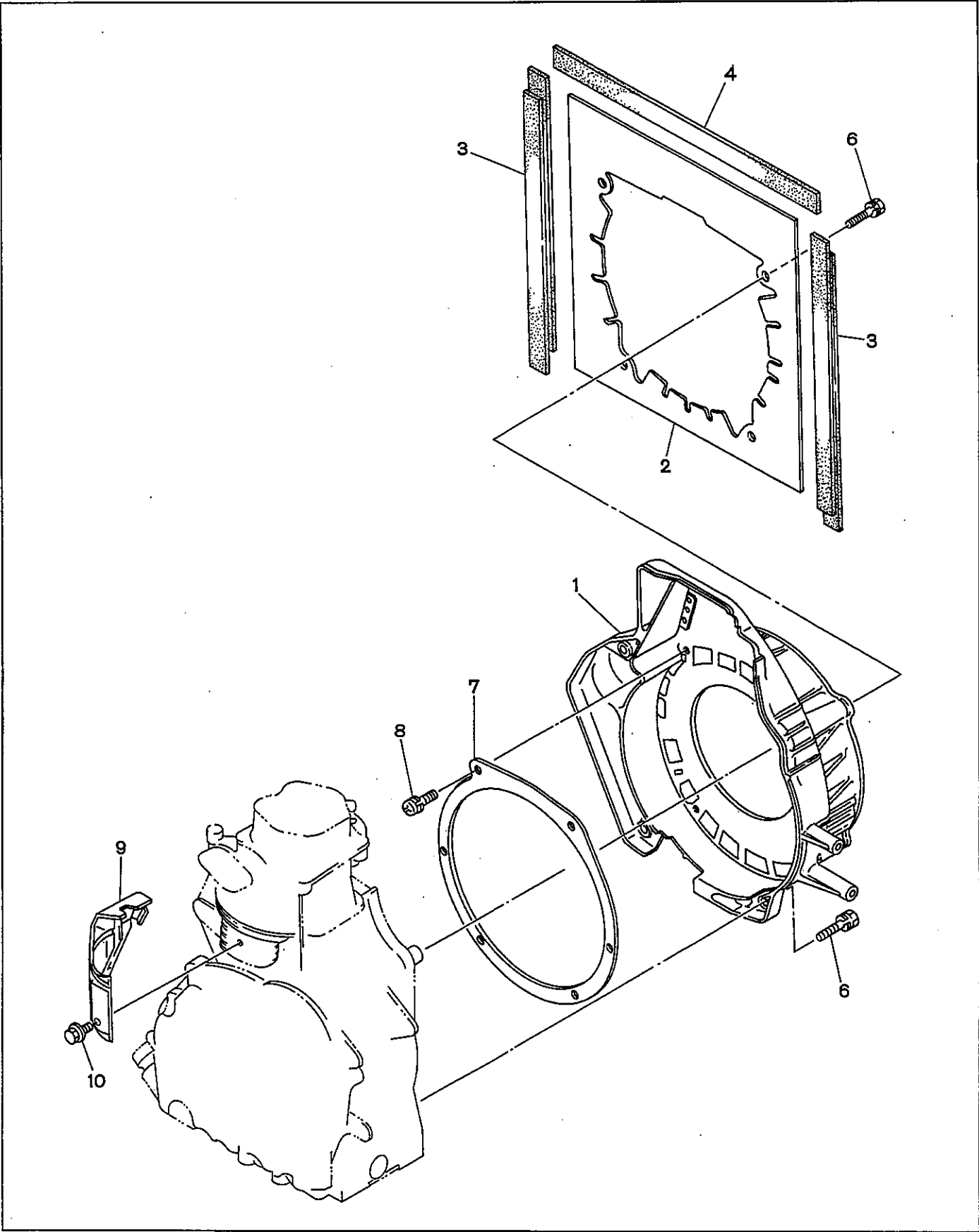
FIG. 13 BLOWER HOUSING
