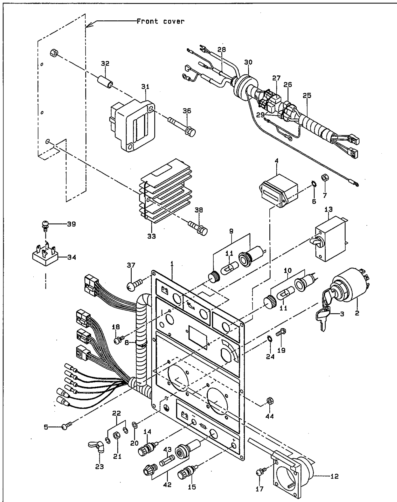
FIG. 3-3 CONTROL PANEL ( GERMANY RECEPTACLE TYPE, 50Hz-230V )
