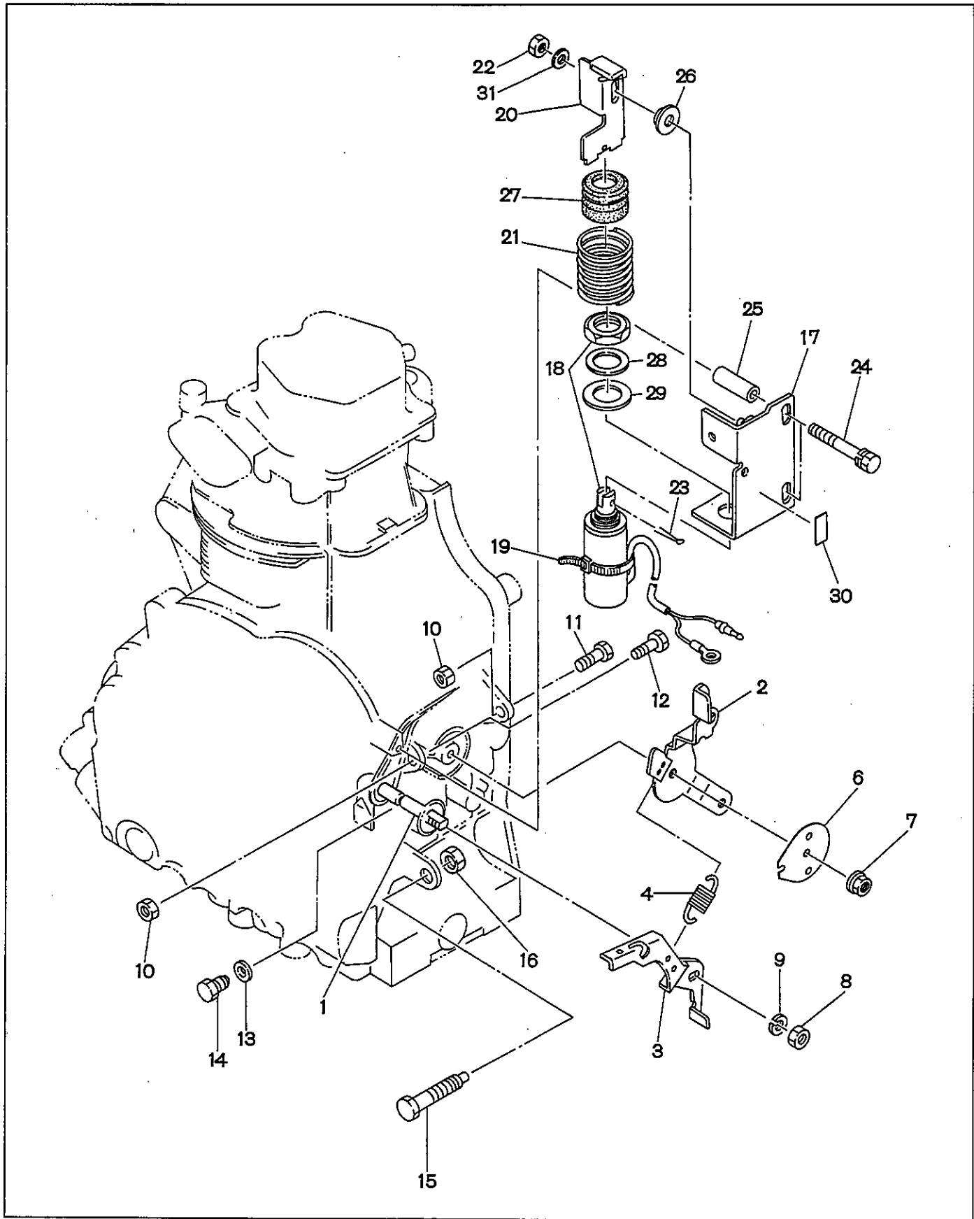
FIG. 12 GOVERNOR OPERATION
