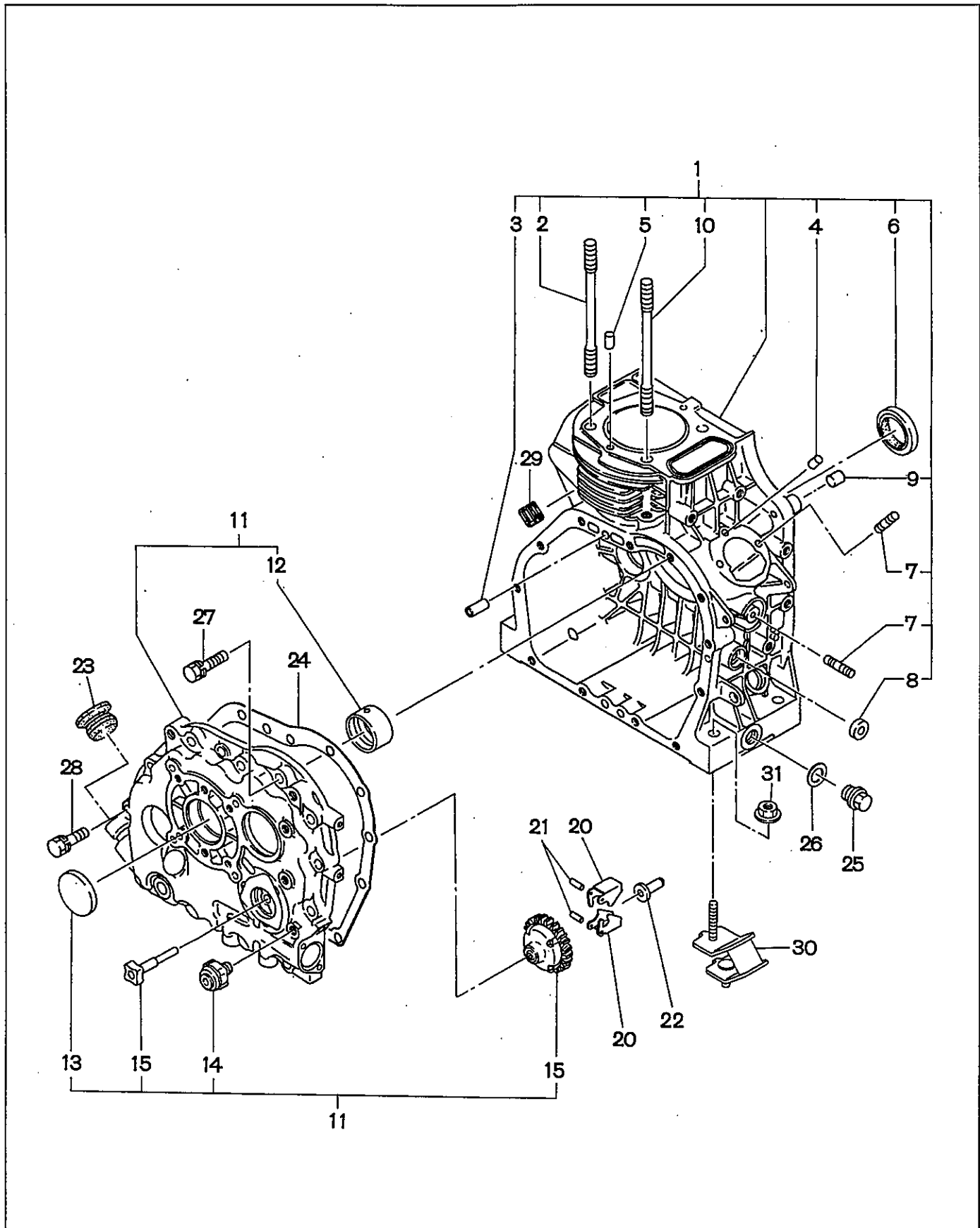
FIG. 7 CRANKCASE
