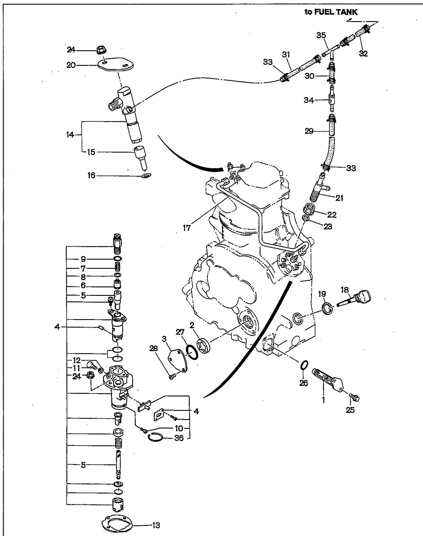
FIG. 14 FUEL SYSTEM
