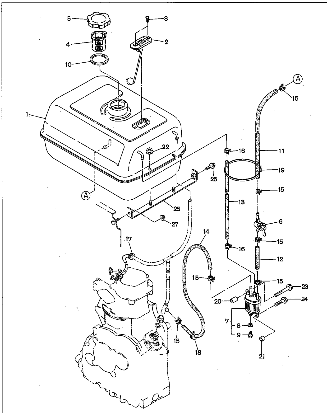
FIG. 5 FUEL TANK
