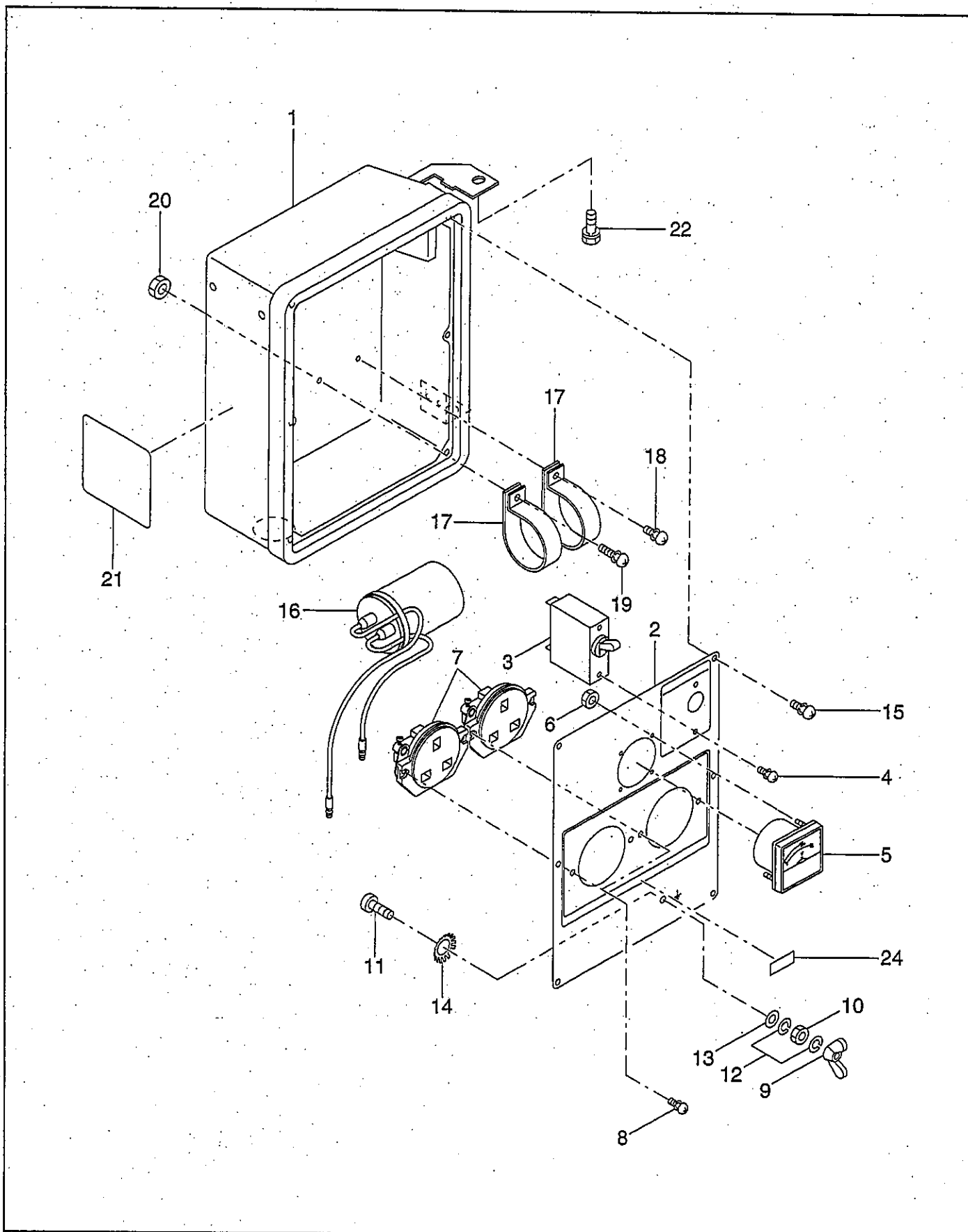
FIG.3 CONTROL BOX (BF RECEPTACLE)
